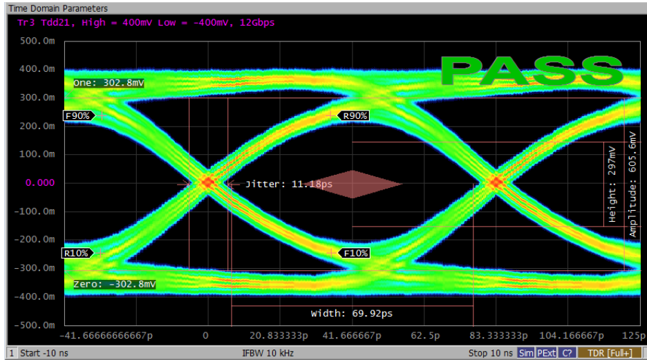
Figure 4. Data Rate 12Gb/s HDMI2.1 Eye Diagram without SY205227DVD
