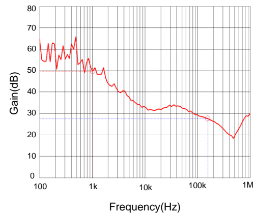
PSRR (V_{IN}=12V, V_{OUT}=3.3V, C_{IN}=Null, C_{OUT}=2.2\mu F, I_{OUT}=300mA)
