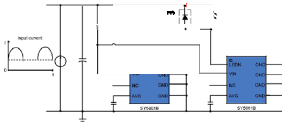
Fig. Parallel circuit
