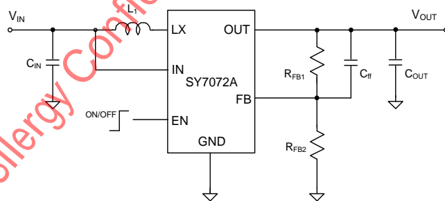
Figure 1. Schematic Diagram
