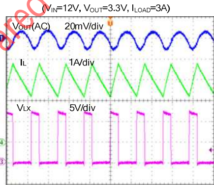
Time (2μs/div)
