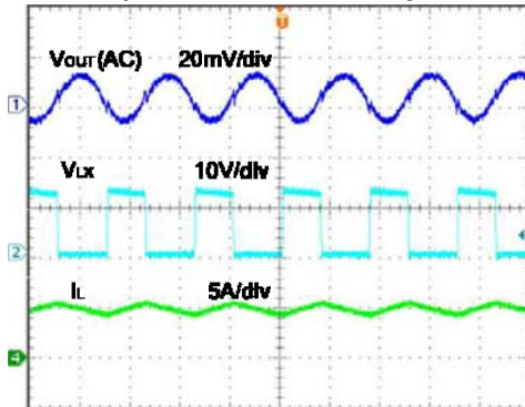
Output Ripple
