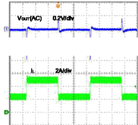
Load Transient
