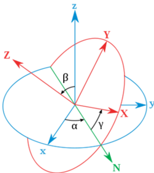
Figure 6.17. Orientation Representation
