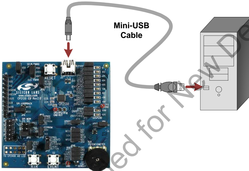
Figure 1. Hardware Setup
