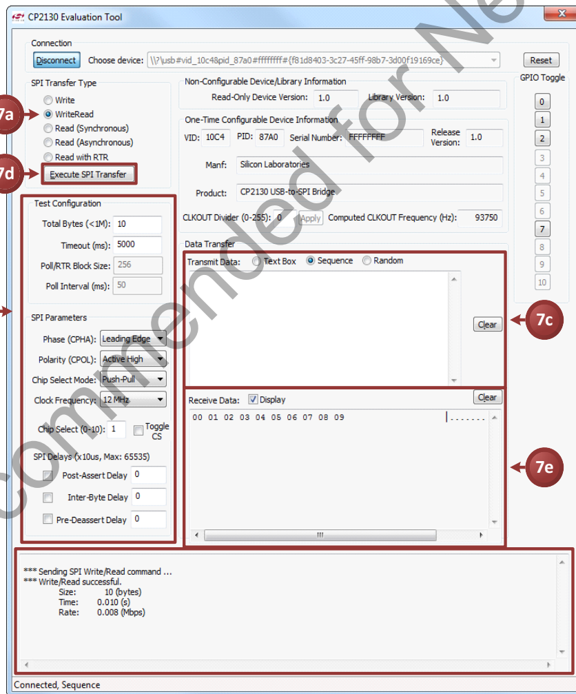
Figure 14. Executing a WriteRead SPI Transfer
