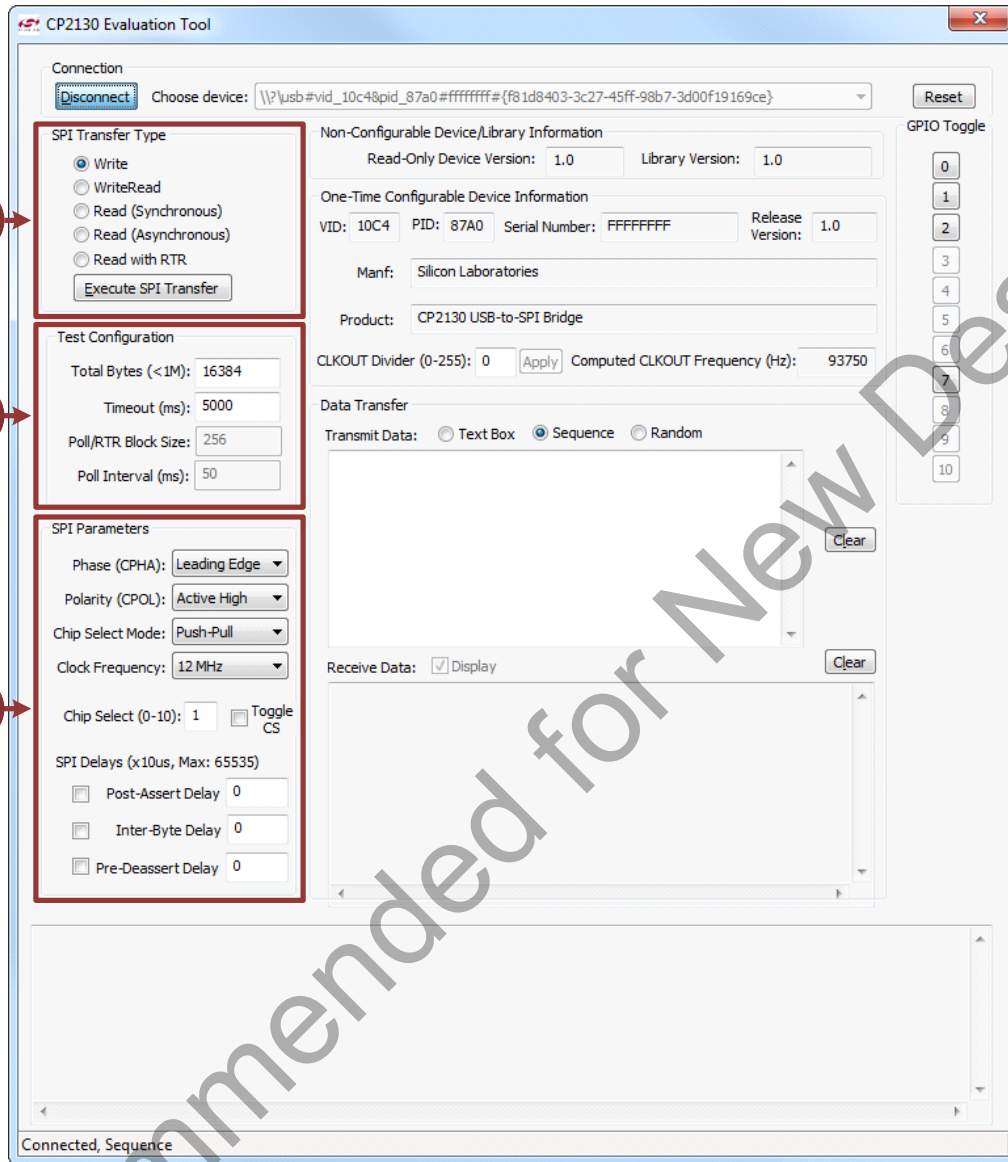
Figure 13. Configuring an SPI Transfer
