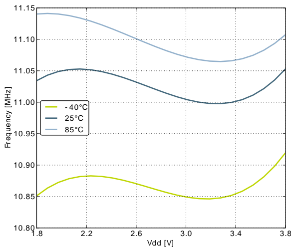
Figure 3.22. Calibrated HFRCO 14 MHz Band Frequency vs Supply Voltage and Temperature
