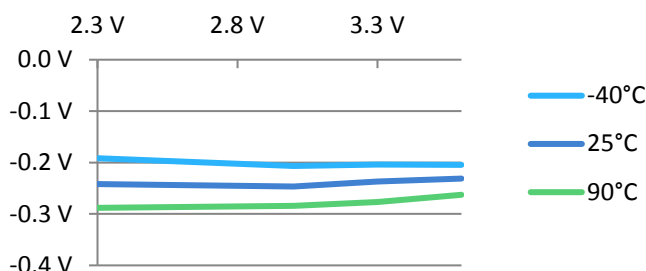
Figure 7: Output Voltage – VDD versus supply voltage when sourcing 8mA
