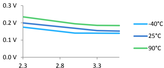
Figure 6: Output Voltage versus supply voltage when sinking 8mA
