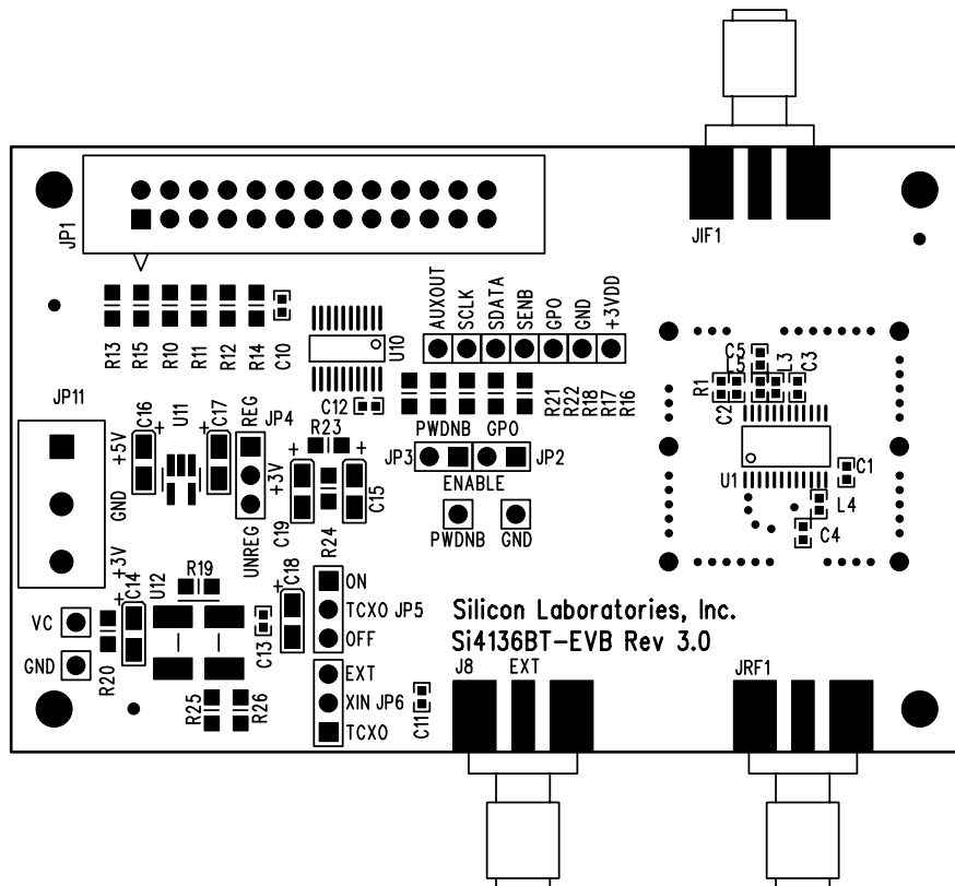
Figure 41. Si4136BT Silkscreen
