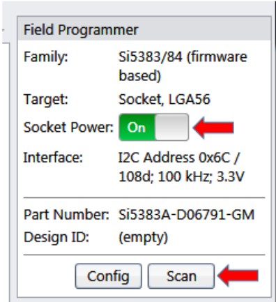
Figure 4.38. In-Socket Scan Prompt and DUT Register Editor Tab
