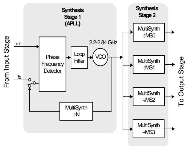
Figure 5. Synthesis Stages
