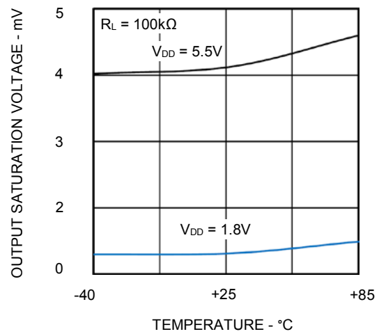
Output Voltage Low ( V_{OL} ) vs Temperature, R_{LOAD} = 100k\Omega
