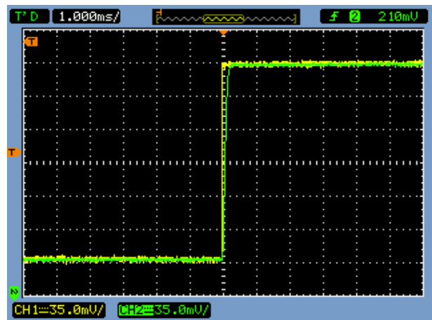
Figure 6: TS1003 Transient Response for R ISO = 50kΩ and C LOAD = 500pF.
