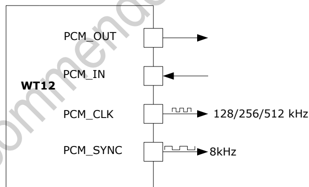
Figure 12: WT12 as PCM master
