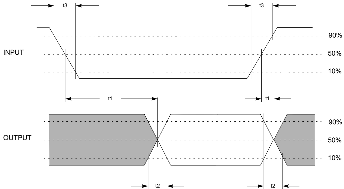
Figure 18-15: USB Timing
