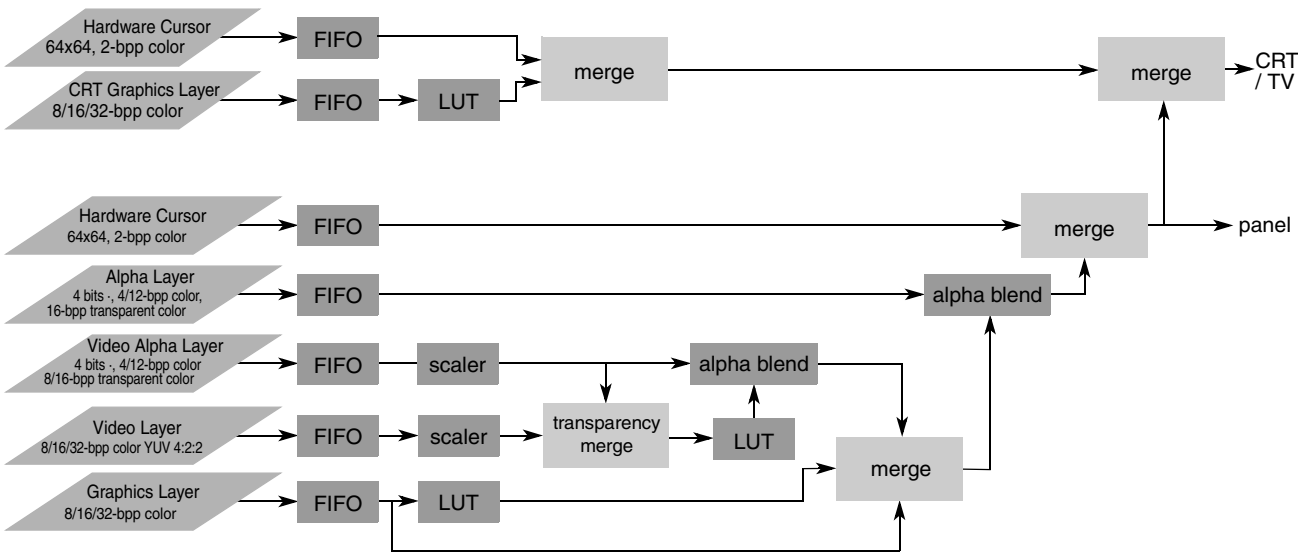
Figure 5-2: Video Layers
