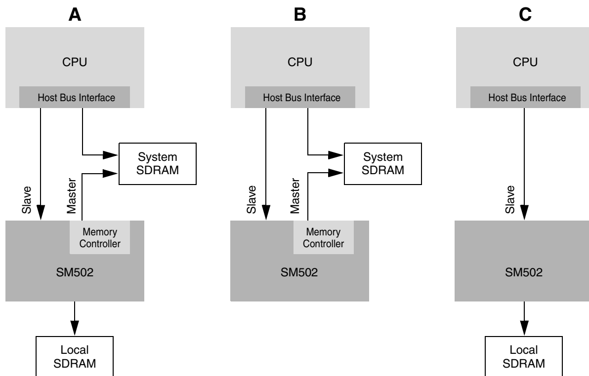
Figure 1-3: System Configurations
