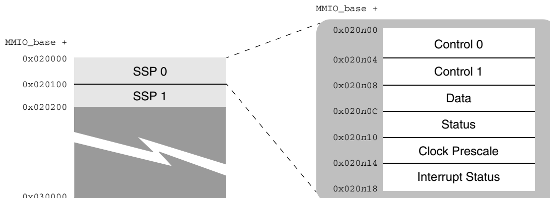
Figure 16-14: Single SSP Register Space
