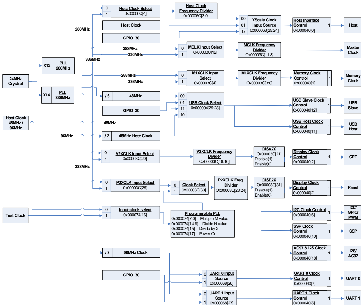
Figure 1-14: Clock Tree
