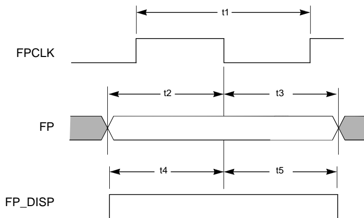
Figure 18-13: FP and FP_DISP Timing
