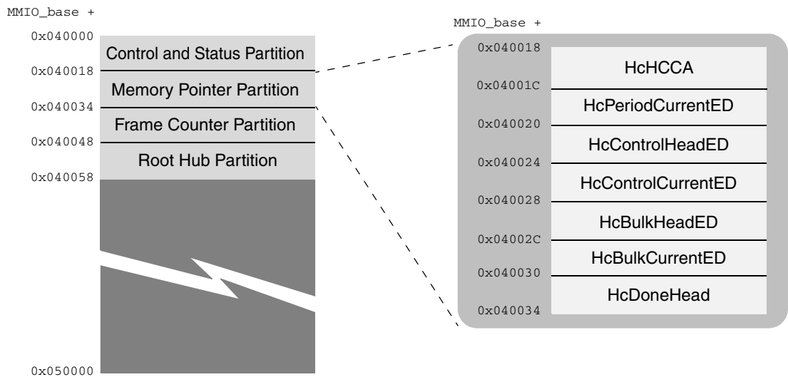
Figure 7-2: USB Memory Pointer Partition Register Space
