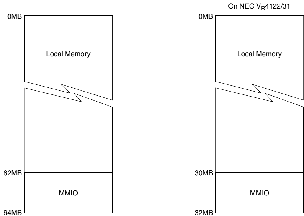
Figure 1-16: Memory Map
