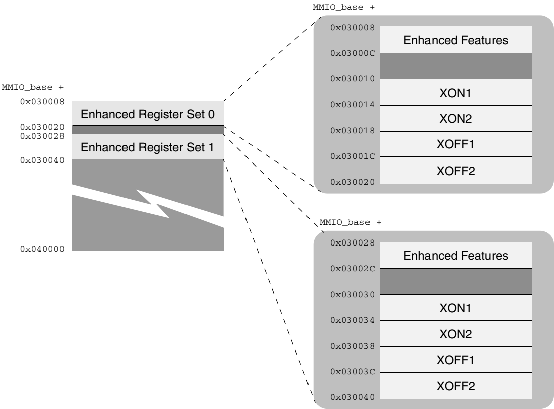
Figure 14-4: Enhanced Register Set
