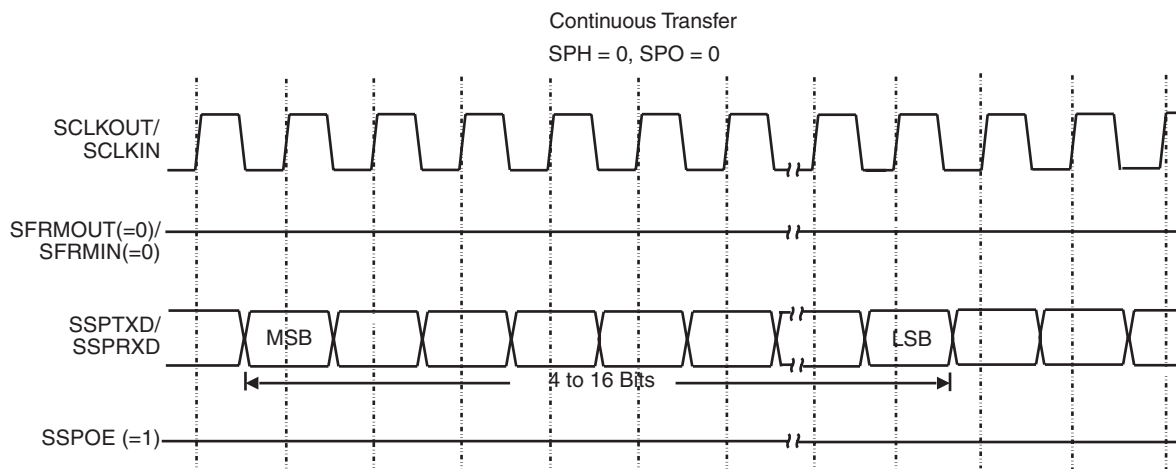
Figure 16-4: Motorola SPI Frame Format (Continuous Transfer) SPO = 0, SPH = 0
