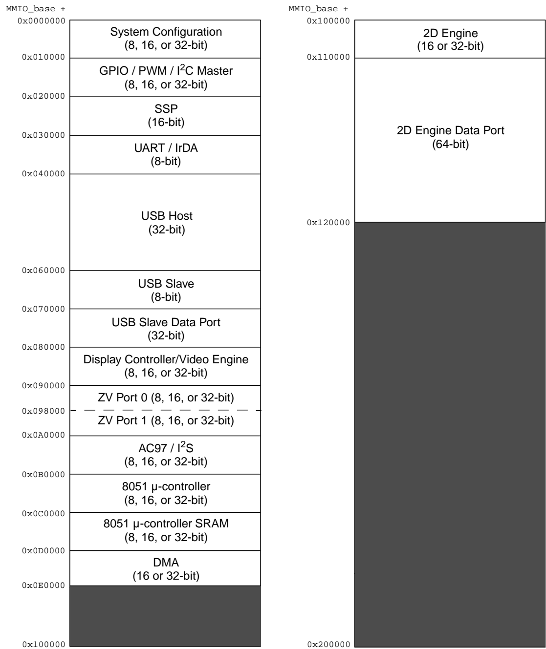
Figure 1-17: MMIO Space
