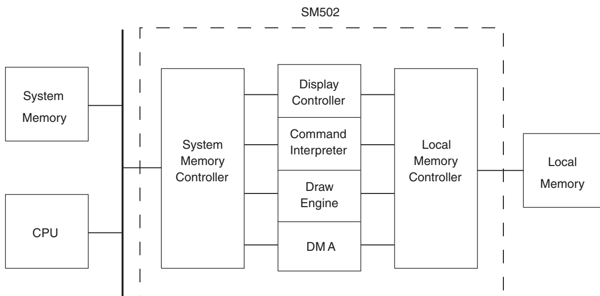
Figure 13-1: SM502 Functional Block Connections to Memory Controllers
