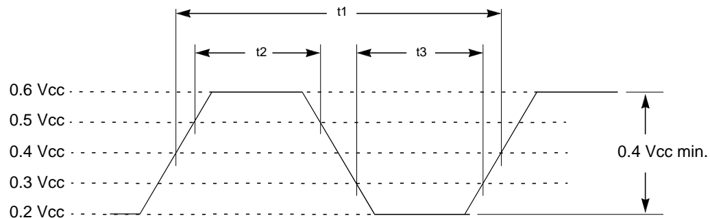
Figure 18-2: PCI Clock Timing
