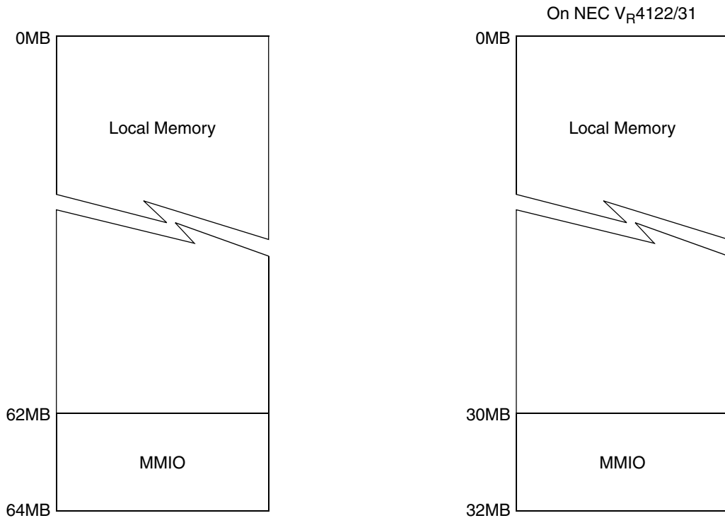
Figure 1-16: Memory Map
