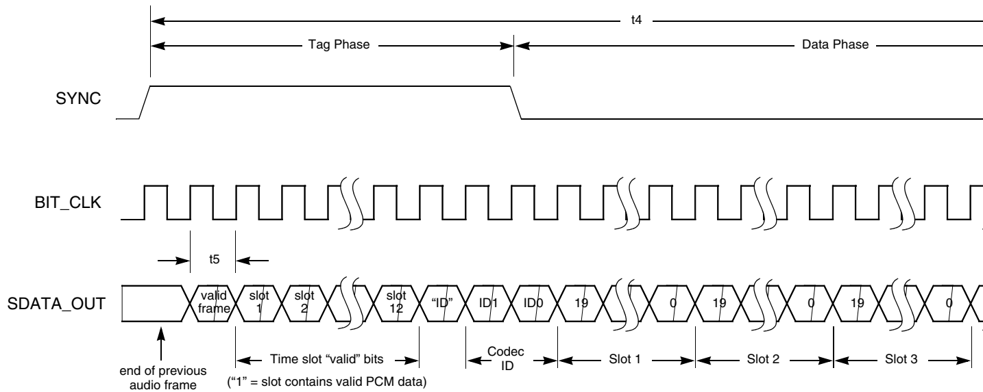
Figure 18-21: AC97-Link Cycle Timing
