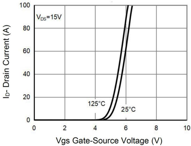
Transfer Characteristics
