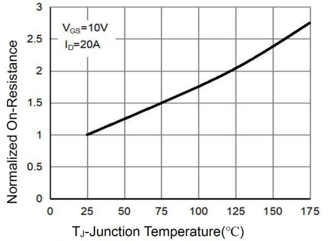
Rdson-Junction Temperature
