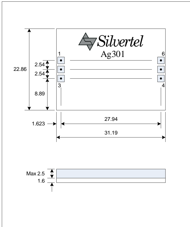
Figure 11: Package Dimensions
