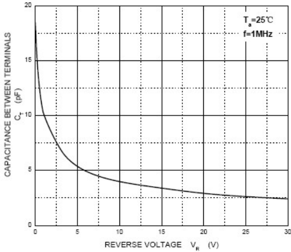
Capacitance Characteristics
