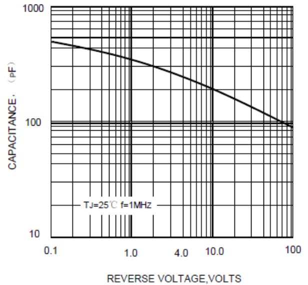
FIG. 4-TYPICAL JUNCTION CAPACITANCE
