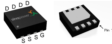
DFN3.3x3.3-8(Saw-EP)
