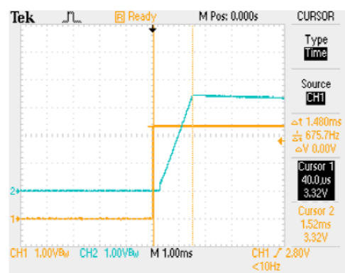
START UP (VIN=5V, VOUT=3.3V)
