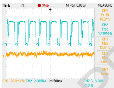
STEADY STATE OPERATION (VIN=5V, VOUT=3.3V, IOUT=100mA)
