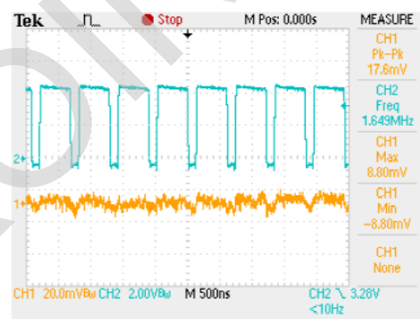
STEADY STATE OPERATION (VIN=5V, VOUT=3.3V, IOUT=1500mA)
