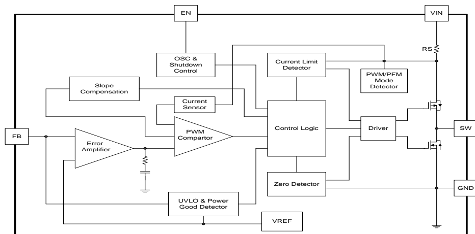
Figure 1. H9008 Block Diagram
