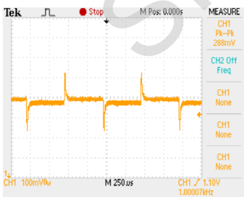
LOAD TRANSIENT RESPONSE (VIN=5V, VOUT=3.3V, IOUT=500-1500mA, 1A/us)
