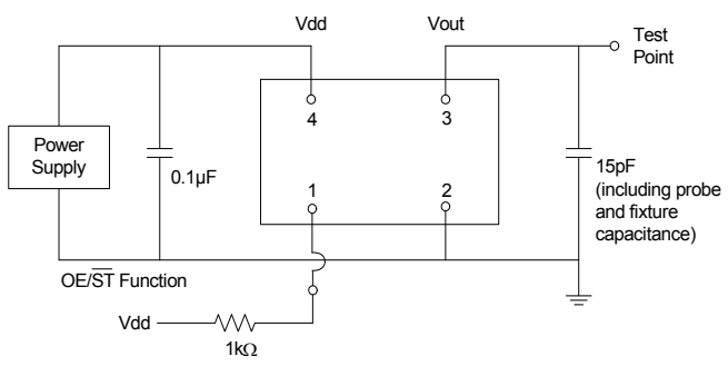
Figure 2. Test Circuit
