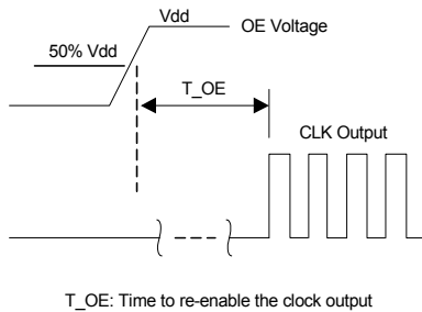
Figure 6. OE Enable Timing (OE Mode Only)
