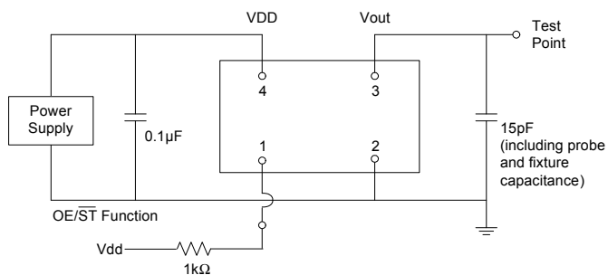
Figure 2. Test Circuit
