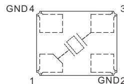
Top View Crystal Connection
