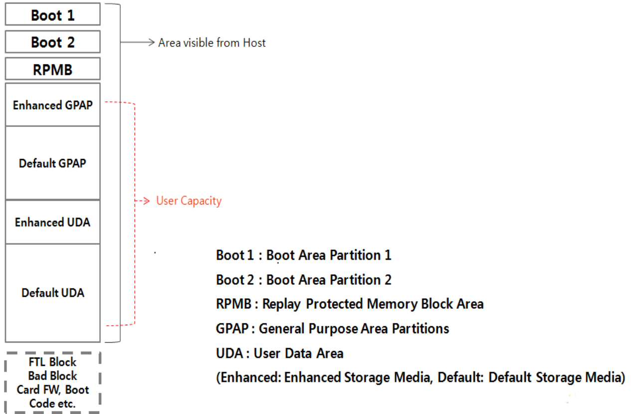
[Figure 21] Partition diagram
