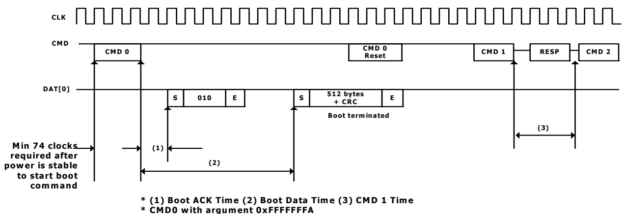
[Figure 23] e-NAND state diagram (Alternative boot mode)
