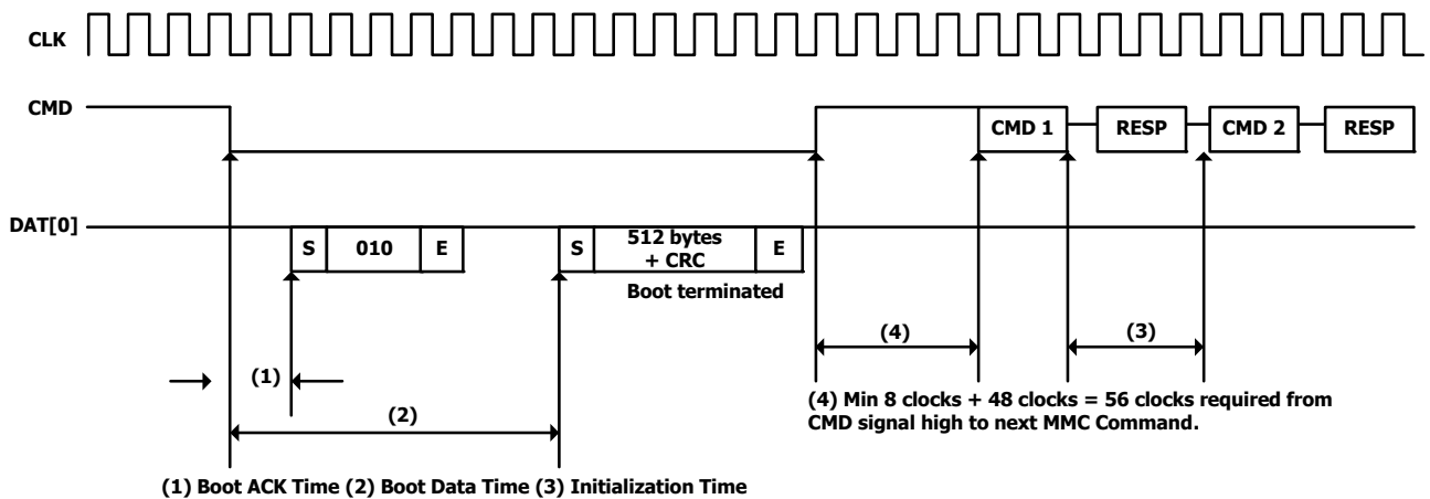
[Figure 22] e-NAND state diagram (Boot mode)
