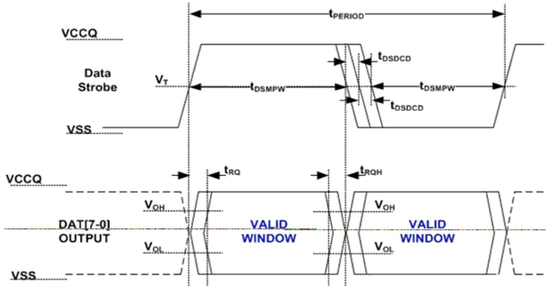
[Figure 4] HS400 Device output timing
