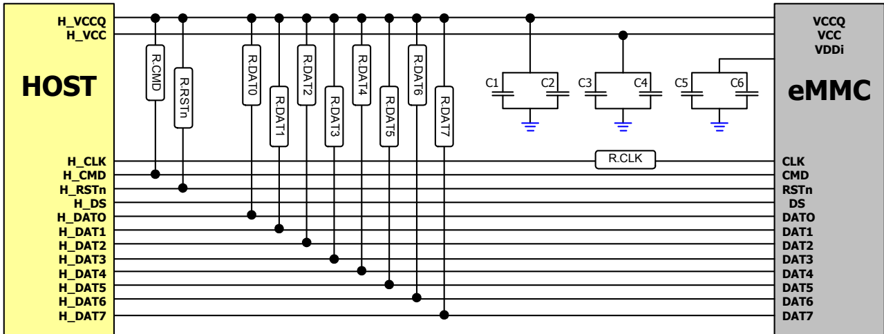
[Figure 20] Connection guide drawing
