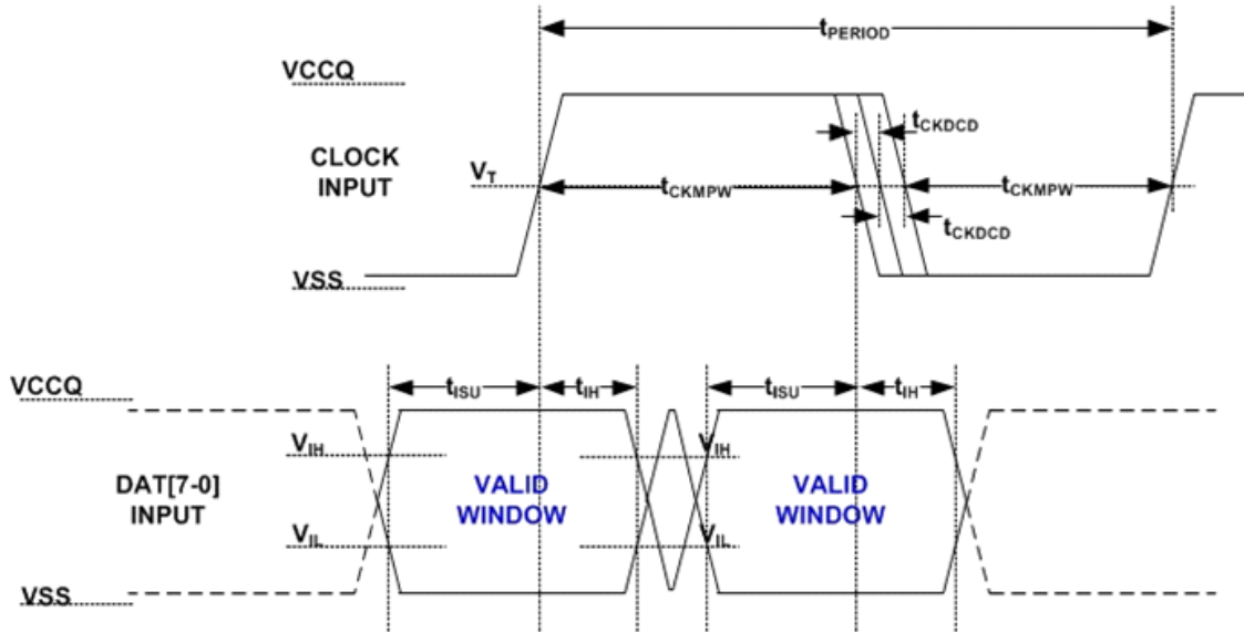
[Figure 3] HS400 Device input timing
