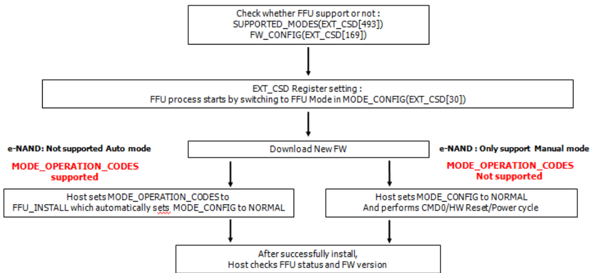
[Figure 7] FFU flow chart
