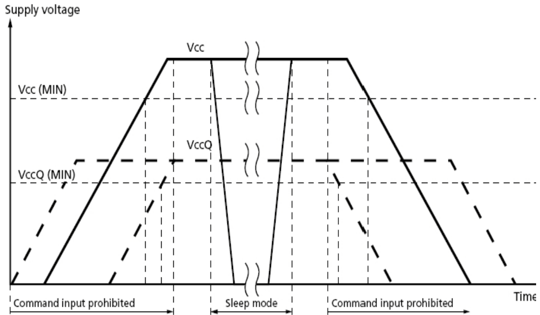
[Figure 18] e-NAND power cycle
