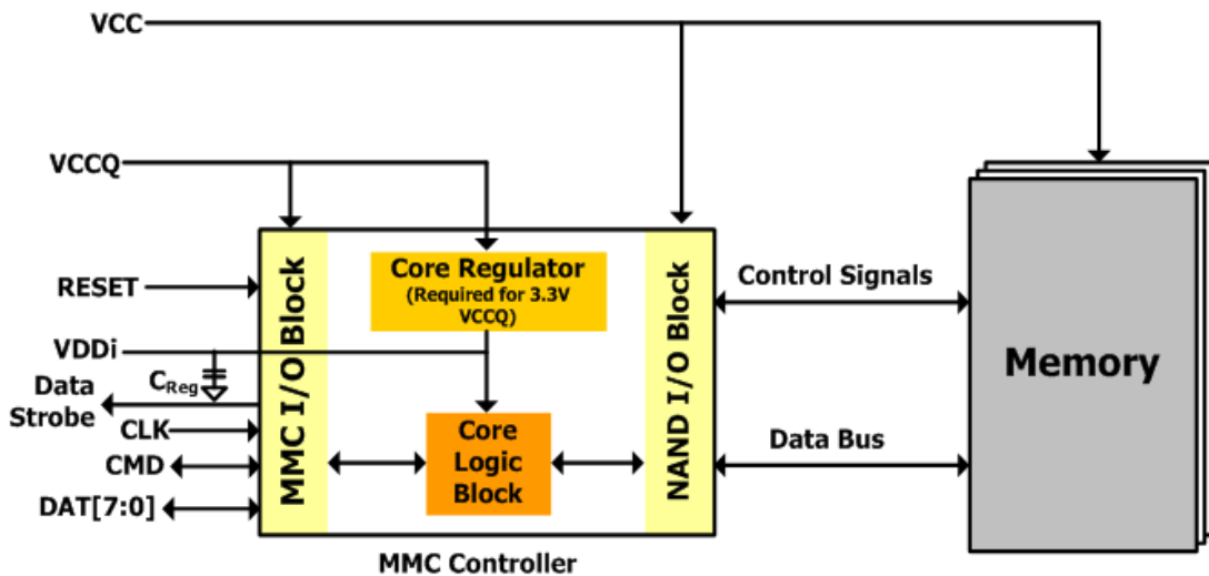
[Figure 19] e-NAND internal power diagram
