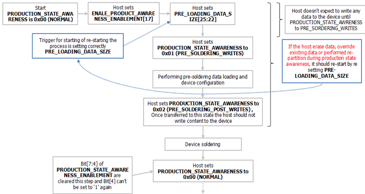
[Figure 8] Production State Awareness manual mode flowchart
