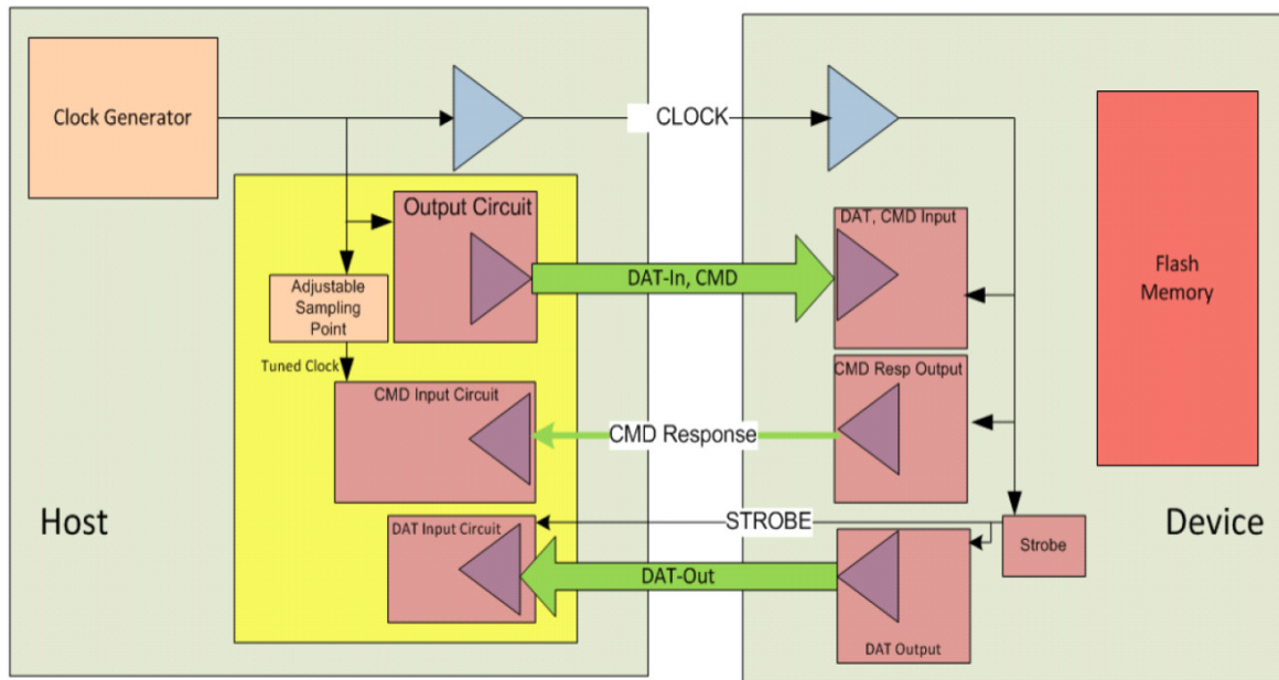
[Figure 5] HS400 Host and Device block diagram
