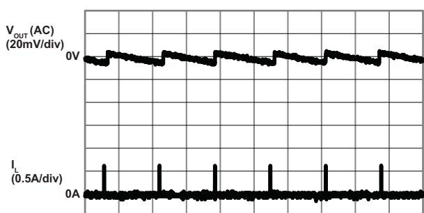
Output Voltage Ripple (V IN = 3.3V; V OUT = 3.8V; L = 2.2μH; I OUT = 0mA)
