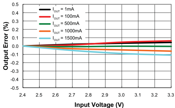
Line Regulation (L = 2.2μH, V OUT = 3.8V)
