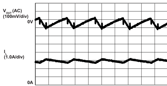
Output Voltage Ripple (V IN = 3.3V; V OUT = 3.8V; L = 2.2μH; I OUT = 2.5A)
