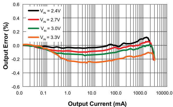
Load Regulation (L = 2.2μH, V OUT = 3.8V)
