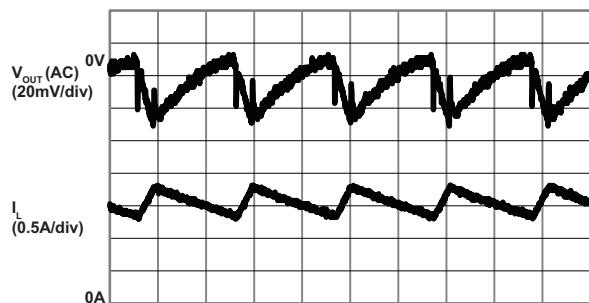
Output Voltage Ripple (V IN = 3.3V; V OUT = 3.8V; L = 2.2μH; I OUT = 1A)
