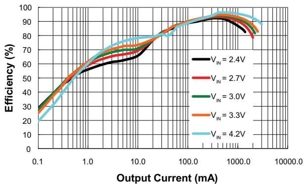
Efficiency (L = 2.2μH, V OUT = 5.0V)
