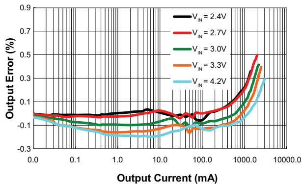
Load Regulation (L = 2.2μH, V OUT = 5.0V)
