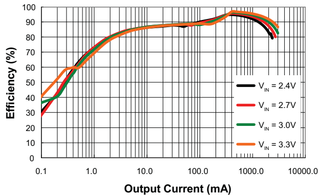
Efficiency (L = 2.2μH, V OUT = 3.8V)
