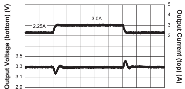
Step-Down Converter Load Transient Response ( I_{OUT} = 2.25A to 3.0A ; V_{IN} = 4.2V ; V_{OUT} = 3.3V ; C_{OUT} = 22\mu F )
