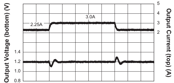
Step-Down Converter Load Transient Response ( I_{OUT} = 2.25A to 3.0A ; V_{IN} = 3.6V ; V_{OUT} = 1.2V ; C_{OUT} = 22\mu F )
