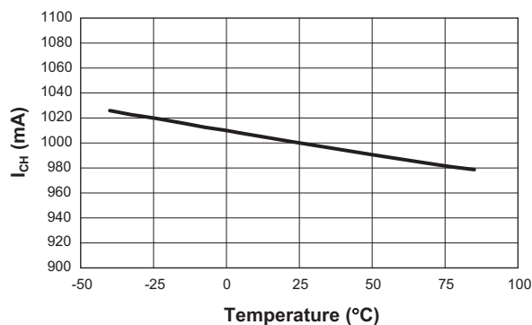
Constant Charging Current vs. Temperature (ADPSET = 8.06kΩ)
