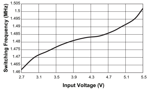
Switching Frequency vs. Input Voltage ( V_{OUTB2} = 1.3V ; I_{OUTB2} = 600mA )
