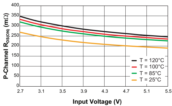
P-Channel R_{DS(ON)} vs. Input Voltage ( V_{OUTB2} = 1.3V )
