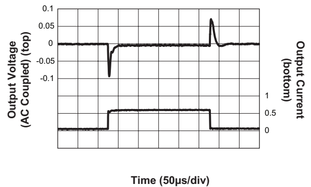
Load Transient ( V_{OUTB2} = 1.3V ; V_{IN} = 3.6V ; I_{OUTB2} = 100mA to 600mA ; C_{FF} = 0pF )
