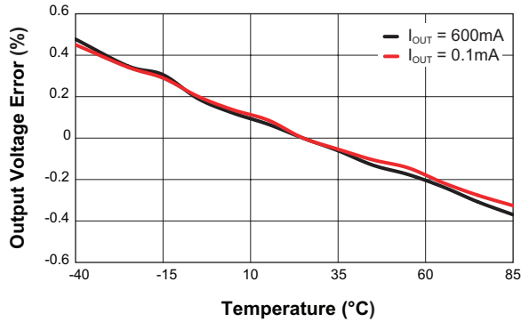
Output Voltage Error vs. Temperature ( V_{OUTB2} = 1.3V ; V_{IN} = 3.6V )
