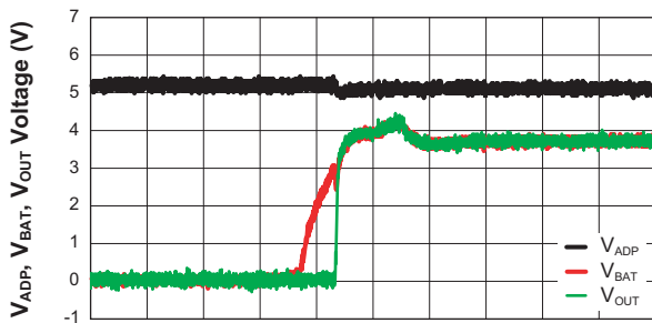
Response of Out when Inserting Battery ( V_{\text{BAT}} = 0\text{V} \rightarrow 3.6\text{V} ; V_{\text{ADP}} = 5\text{V} ; V_{\text{ENB\text{AT}}} = 5\text{V} ; V_{\text{ENO}} = 0\text{V} ; R_{\text{LOAD}} = 50\Omega )
