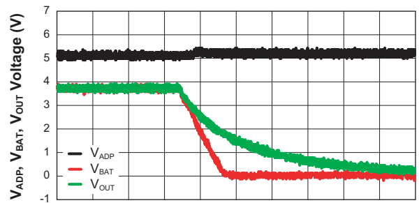
Response of Out when Removing Battery ( V_{\text{BAT}} = 3.6\text{V} \rightarrow 0\text{V} ; V_{\text{ADP}} = 5\text{V} ; V_{\text{ENB\text{AT}}} = 5\text{V} ; V_{\text{ENO}} = 0\text{V} ; R_{\text{LOAD}} = 50\Omega )
