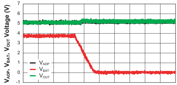
Response of Out when V_{ENB\text{AT}} = 0\text{V} ( V_{\text{BAT}} = 3.6\text{V} \rightarrow 0\text{V} ; V_{\text{ADP}} = 5\text{V} ; V_{\text{ENO}} = 5\text{V} ; R_{\text{LOAD}} = 50\Omega )
