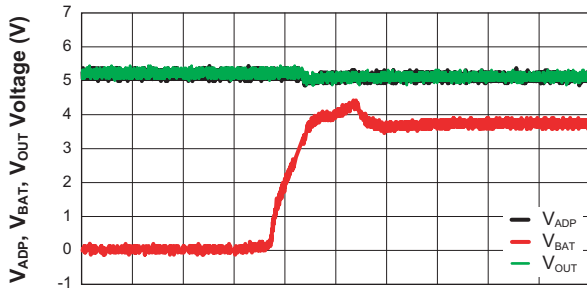
Response of Out when V_{ENB\text{AT}} = 0\text{V} ( V_{\text{BAT}} = 0\text{V} \rightarrow 3.6\text{V} ; V_{\text{ADP}} = 5\text{V} ; V_{\text{ENO}} = 5\text{V} ; R_{\text{LOAD}} = 50\Omega )
