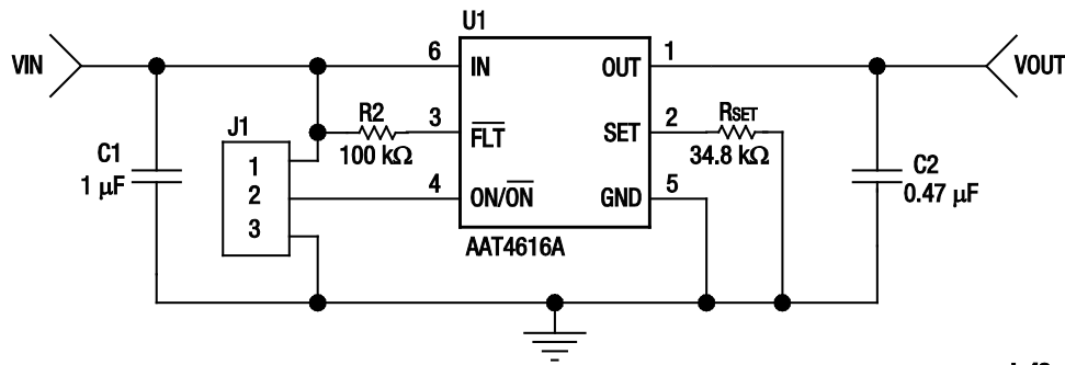
Figure 17. AAT4616A Evaluation Board Schematic
