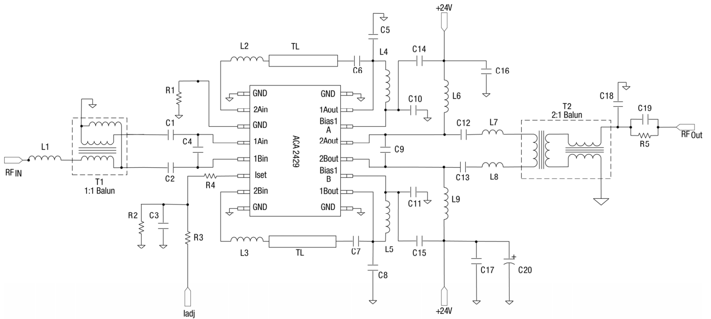
Figure 3. ACA2429 Evaluation Board Schematic
