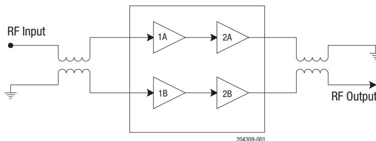
Figure 1. ACA2429 Block Diagram
