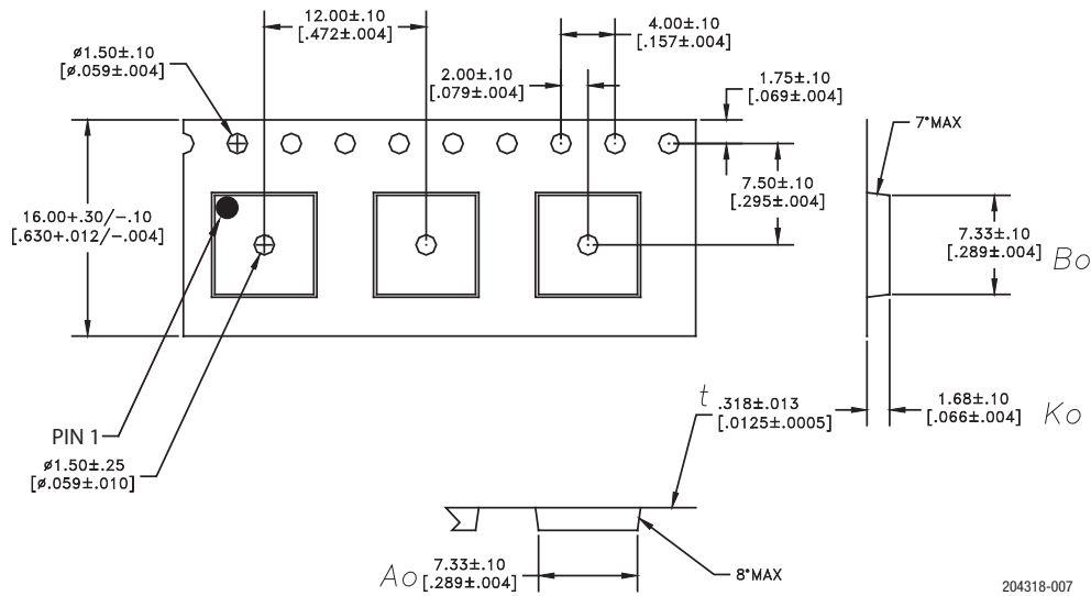
Figure 7. AWB7231 Tape and Reel Dimensions
