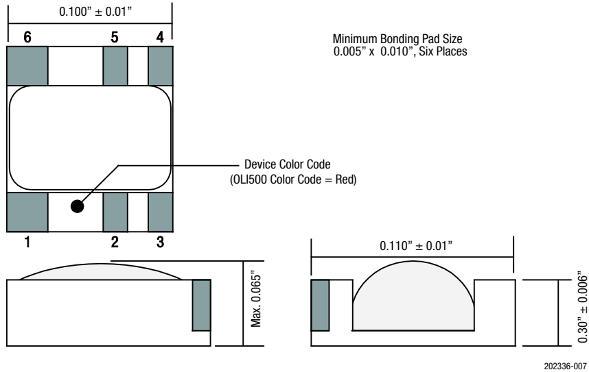
Figure 7. OLI500 Package Dimensions
