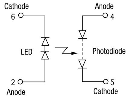
Figure 1. OLS910 Block Diagram
