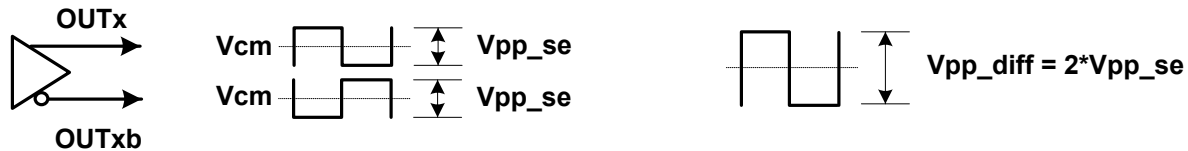
Differential Output Test Configuration
