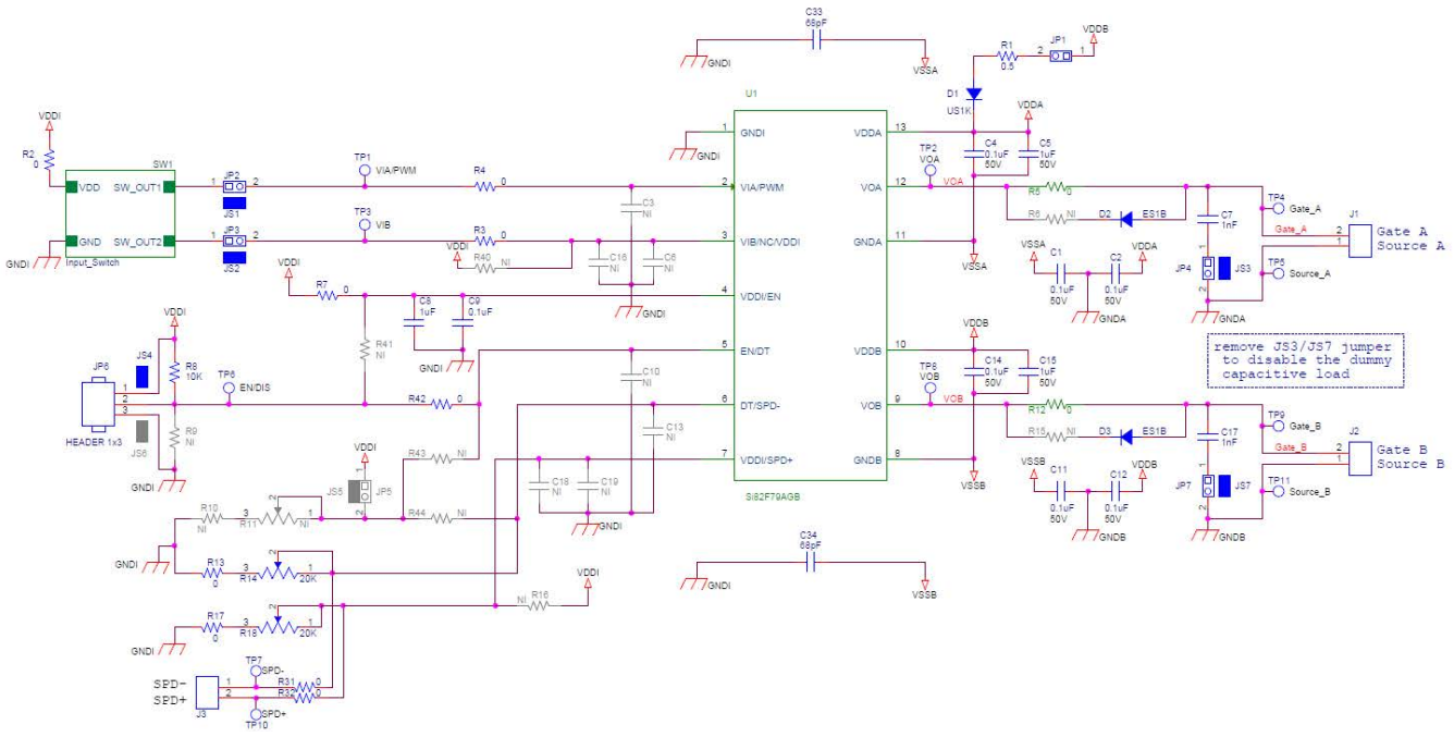
Figure 16. Si82Fx Driver (LGA-13 Package)
