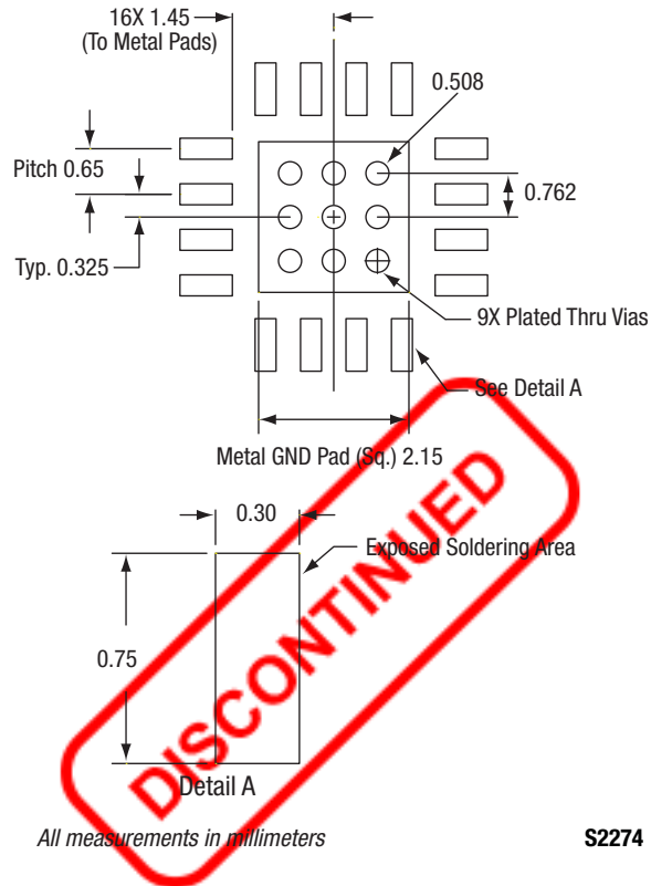
Figure 25. SKY12208-306LF PCB Layout Footprint
