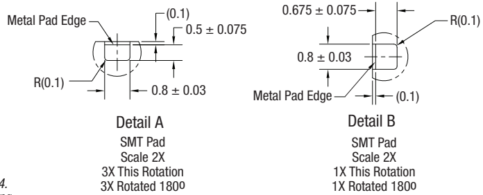
Figure 13. SKY12236-11 Package Dimensions
