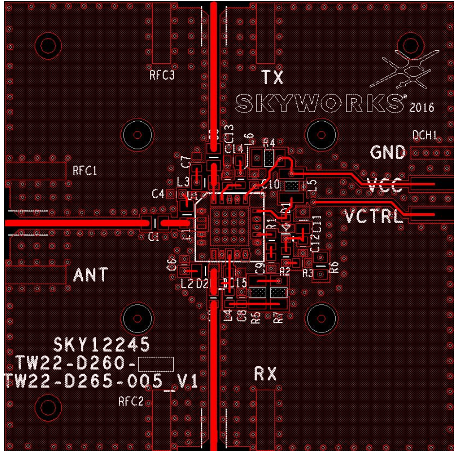
Figure 25. SKY12245-492LF Evaluation Board Assembly Diagram
