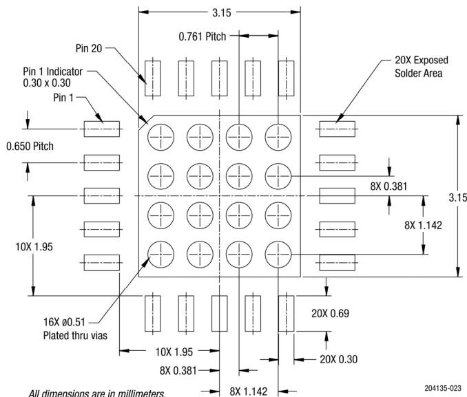
Figure 27. PCB Layout Footprint
