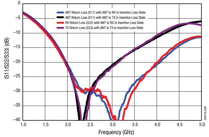
Figure 8. Return Loss vs Frequency
