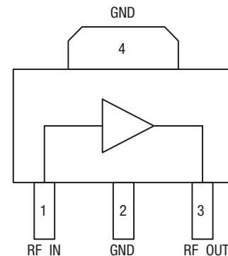
Figure 1. SKY65009-70LF Functional Block Diagram
