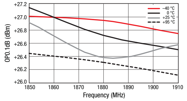
Figure 44. OP0.1dB vs Frequency Over Temperature
