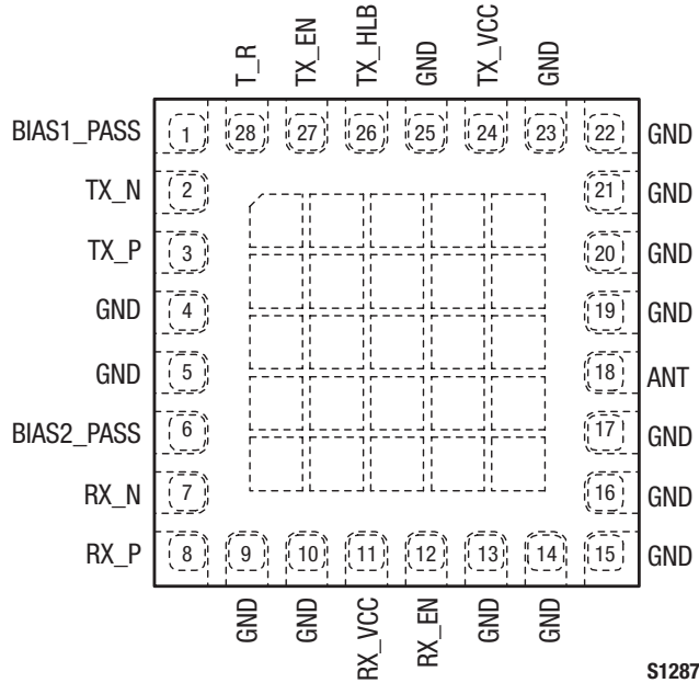
Figure 2. SKY65336-11 Pinout (Top View)
