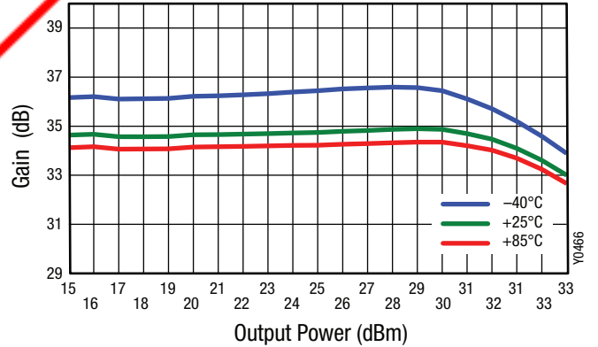
Figure 6. Gain vs Output Power over Temperature
