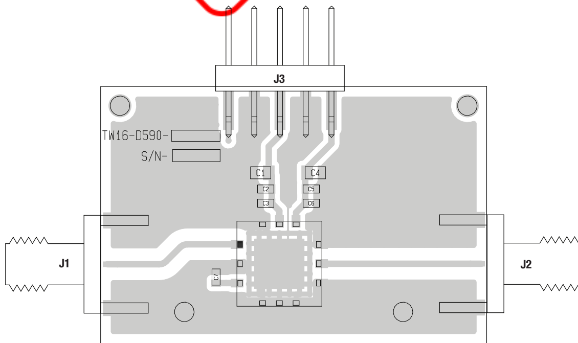
Figure 4. SKY65388-11 Evaluation Board Assembly Drawing
