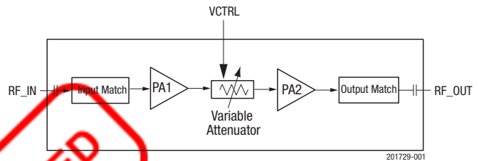
Figure 1. SKY65388-11 Block Diagram
