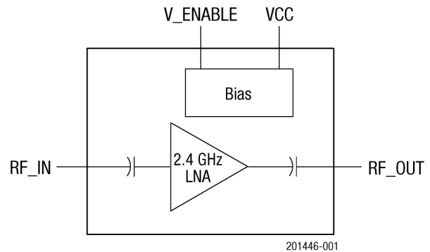
Figure 1. SKY65405-21 LNA Block Diagram
